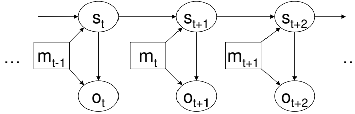
Fig. 2. A portion of a Bayesian Network representing the POMDP model. Decisions are drawn in a rectangle to show that they are actions of the system rather than observed random variables.
