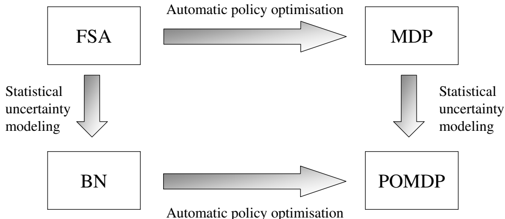
Fig. 1. Frameworks for modelling uncertainty and policy optimisation in Spoken Dialogue Systems: Finite State Automata (FSA), Bayesian Networks (BN), Markov Decision Processes (MDP) and Partially Observable MDPs (POMDP).
