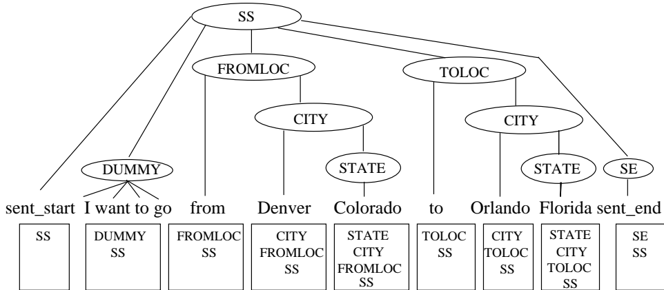
Fig. 3. Example of a Parse Tree and its Vector State Equivalent.
