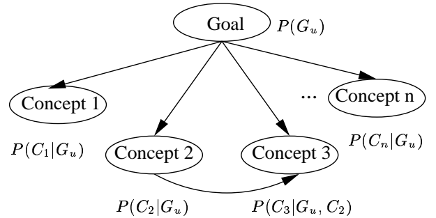
Fig. 4. Example of a Tree-Augmented Naive Bayes Network.
