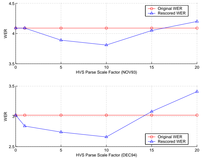
Fig. 6. Scale of semantic parse score vs WER.
