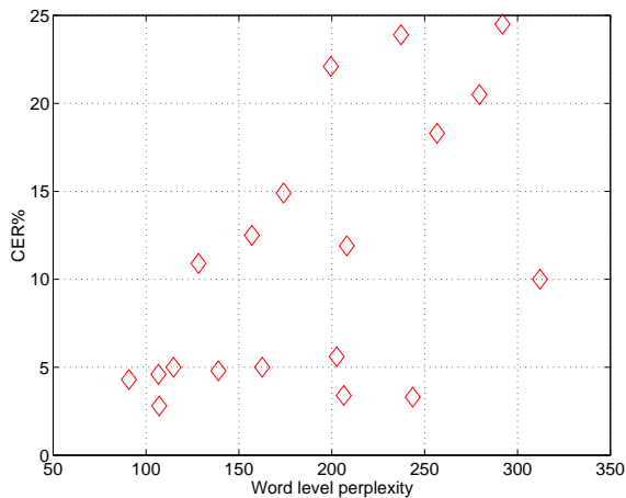
Fig. 2. Correlation between word level perplexity and CER
