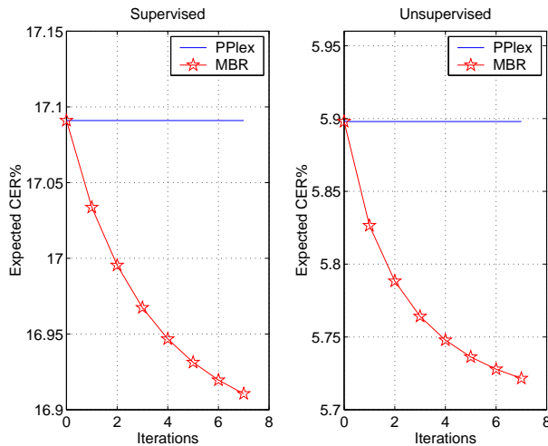
Fig. 1. MBR criterion on bnmdev06, bcmdev05 and eval06 for supervised and unsupervised adapted LMs using PP and MBR.
