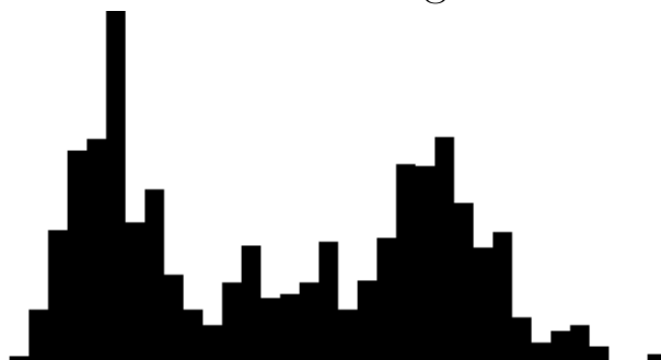
Orientation Histogram
