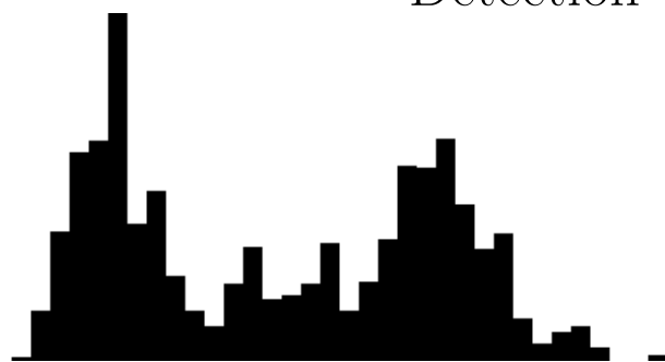
Orientation Histogram
