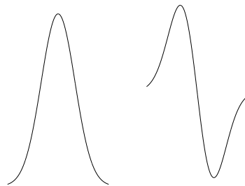
g_\sigma(x) g'_\sigma(x)
