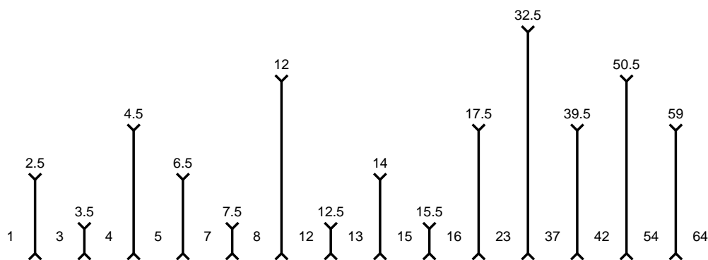
A metric tree in 1 dimension
