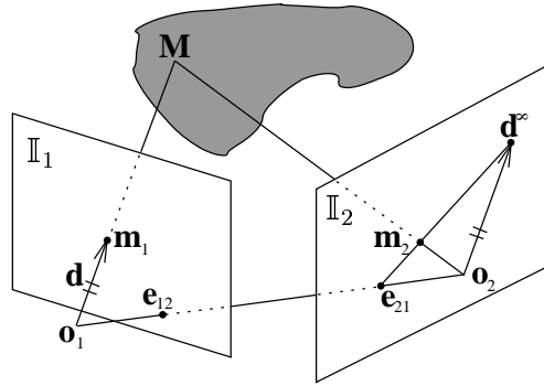
Figure 2.11: Epipolar geometry.
