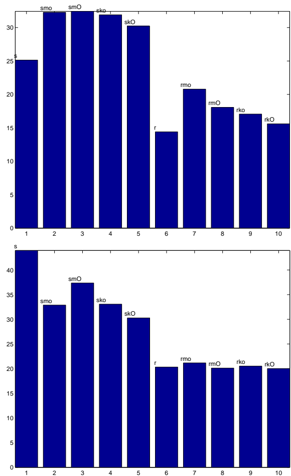
Figure 2: The perplexities of 10 different LSA indexing methods. The upper picture shows perplexities when 50 best cluster models ( k=50 ) are used for the smoothing and the lower picture when the match is approximated by only the best cluster model ( k=1 ). The explanation of the method ids: ‘s’ = SVD, ‘m’ = SOM, ‘o’ = 260 clusters, ‘O’ = 2000 clusters and ‘k’ = SOM0.
